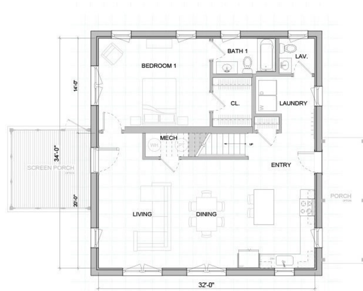
FIRST FLOOR
