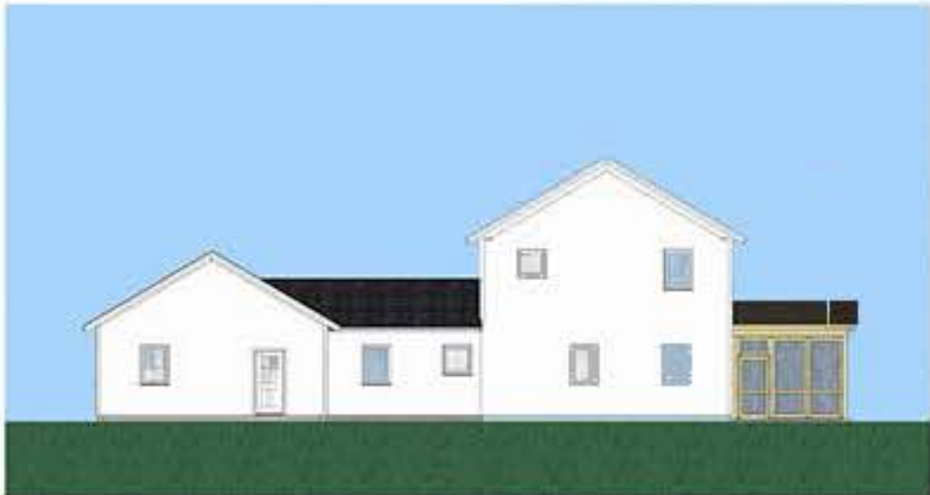
BACK ELEVATION
