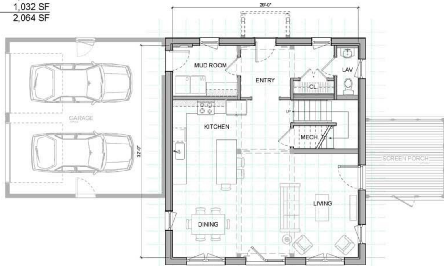
FIRST FLOOR
