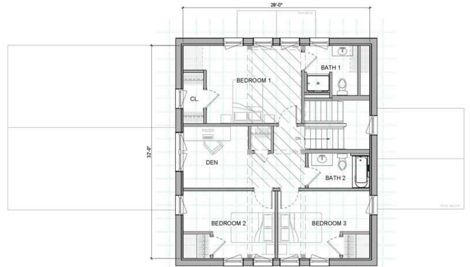
SECOND FLOOR
